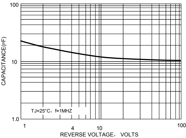
FIG.5-TYPICAL JUNCTION CAPACITANCE
