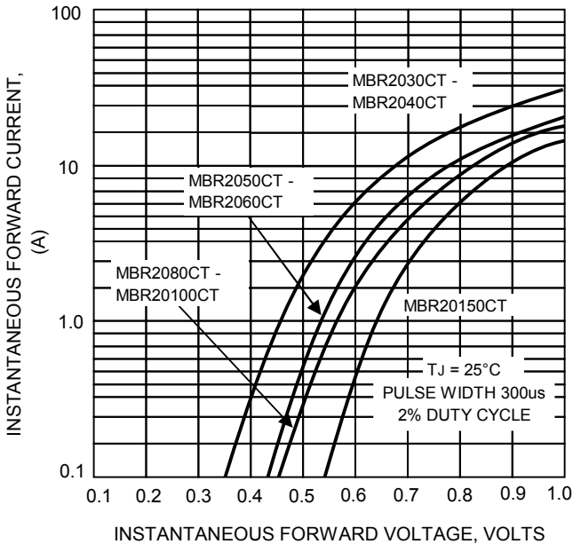
FIG.4-TYPICAL FORWARD CHARACTERISTICS
