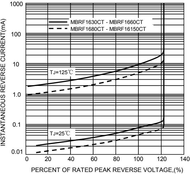
FIG.3-TYPICAL REVER CHARACTERISTICS
