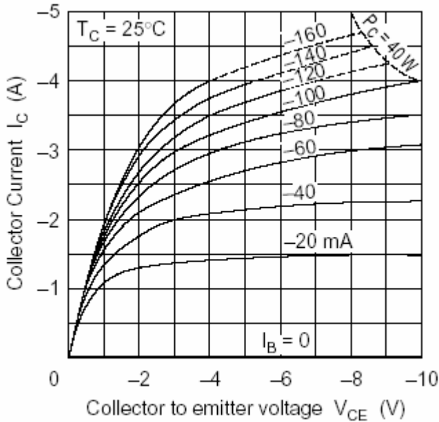
Fig.3 Static Characteristic
