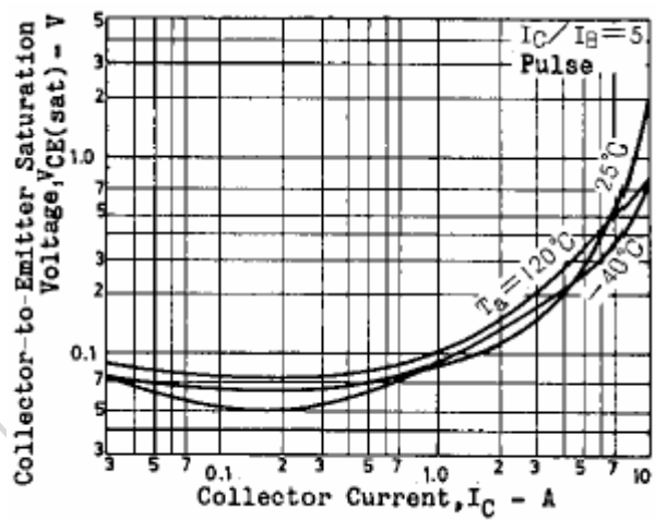
Fig.6 Collector-Emitter Saturation Voltage
