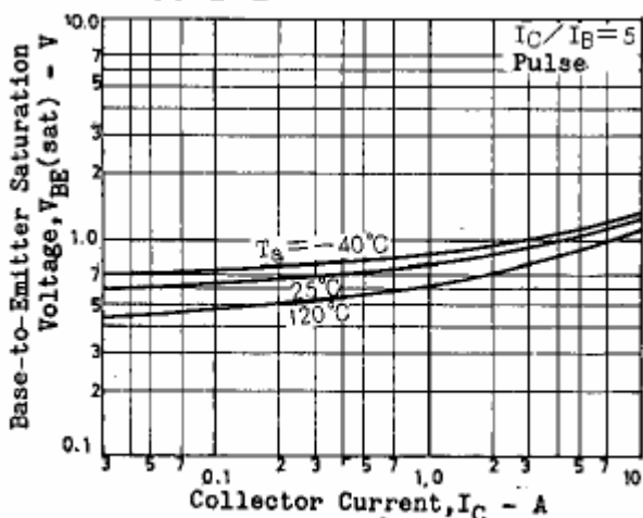
Fig.7 Base-Emitter Saturation Voltage
