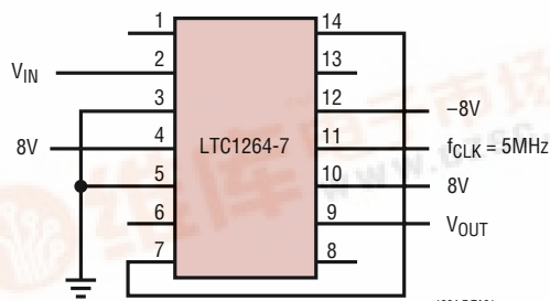
200kHz Linear Phase Lowpass Filter
