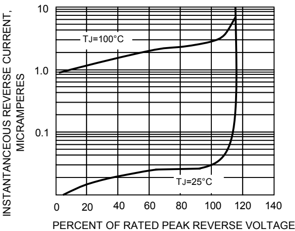
FIG.4-TYPICAL REVERSE CHARACTERISTICS
