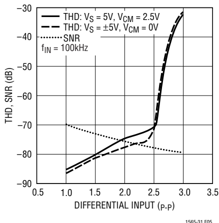
Figure 5. Dynamic Range Diff-In, Diff-Out
