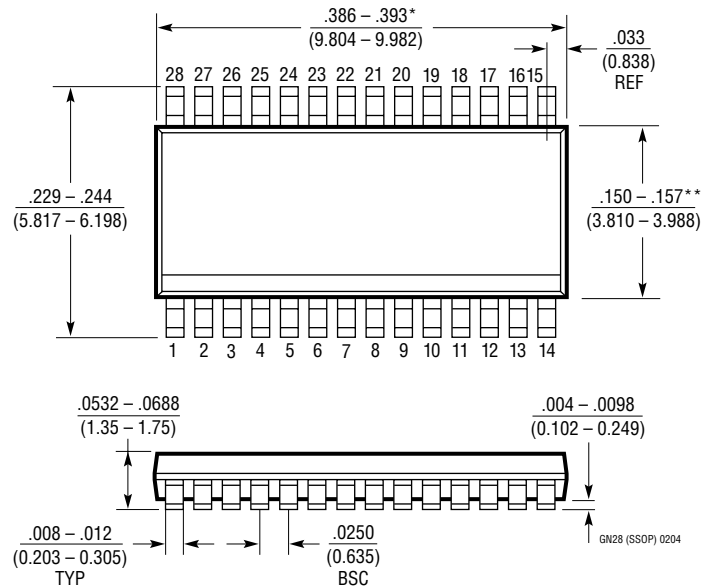
GN Package 28-Lead Plastic SSOP (Narrow 0.150) (LTC DWG # 05-08-1641)
