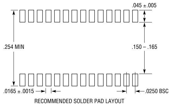
GN Package 28-Lead Plastic SSOP (Narrow 0.150) (LTC DWG # 05-08-1641)
