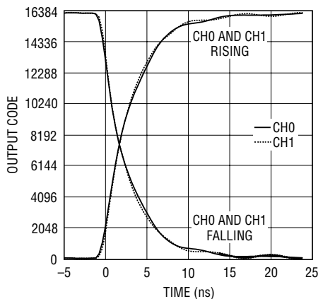
Output Match with Simultaneous Input Steps at CH0 and CH1 from 25\Omega
