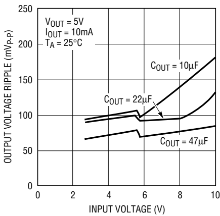
LTC1514-5 Output Voltage Ripple vs Input Voltage
