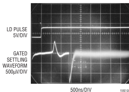
Full-Scale Settling Waveform
