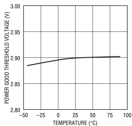
Power Good Threshold Voltage vs Temperature ( 3V_{OUT} )
