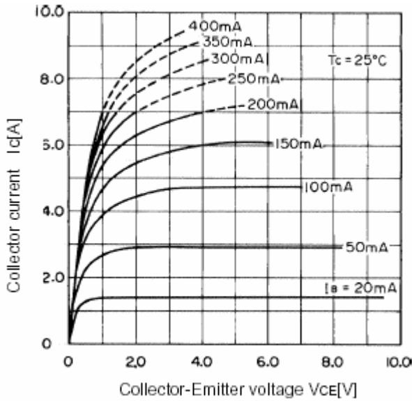
Fig.3 Static Characteristic
