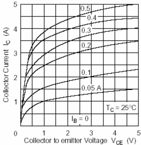
Fig.3 Static Characteristic
