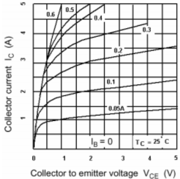
Fig.4 Static Characteristic
