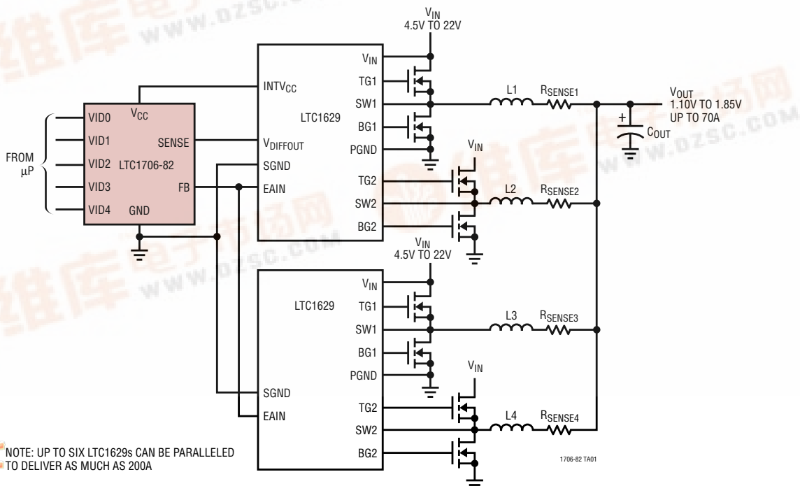
VID Controlled High Current 4-Phase DC/DC Converter (Simplified Block Diagram)
