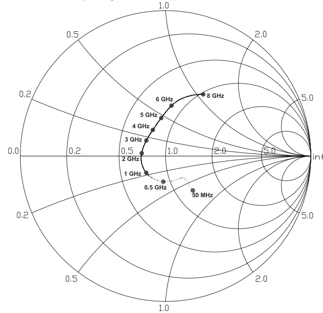
S11 versus Frequency (5V 46mA)
