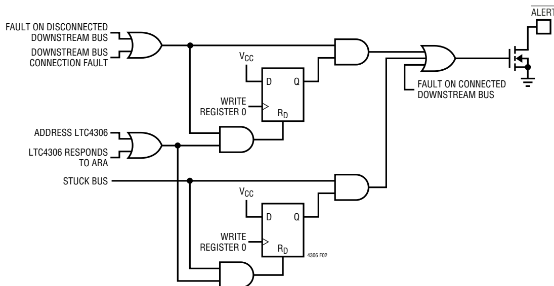
Figure 2. Setting and Resetting the \overline{\text{ALERT}} Pin
