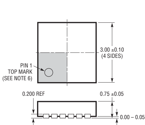
DD Package 12-Lead Plastic DFN (3mm × 3mm) (Reference LTC DWG # 05-08-1725 Rev A)
