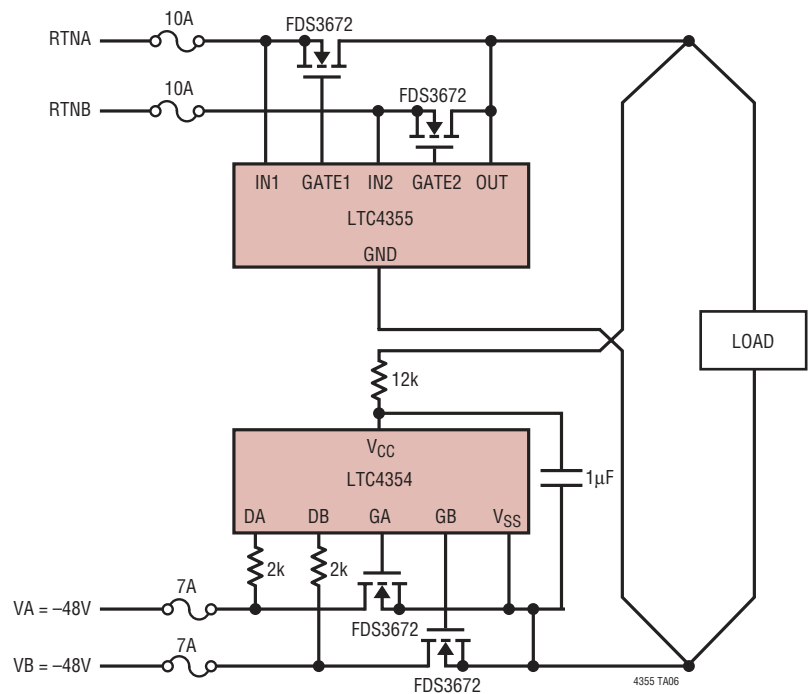
200W AdvancedTCA Ideal Diode-OR
