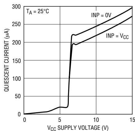
V_{\text{CC}} Supply Quiescent Current vs Voltage
