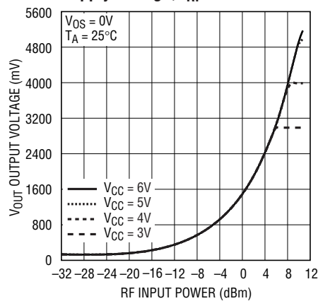
V_{OUT} vs RF Input Power and V_{CC} Supply Voltage, f_{RF} = 1000\text{MHz}
