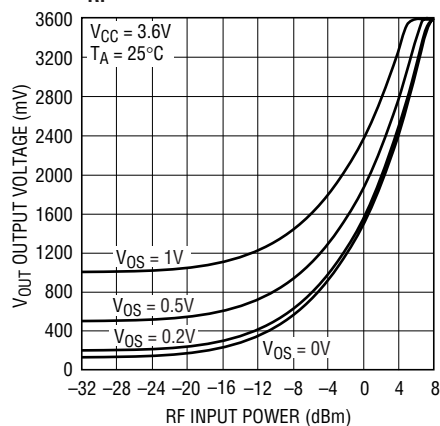
V_{OUT} vs RF Input Power and V_{OS} , f_{RF} = 1000\text{MHz}
