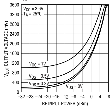
V_{OUT} vs RF Input Power and V_{OS} , f_{RF} = 300\text{MHz}
