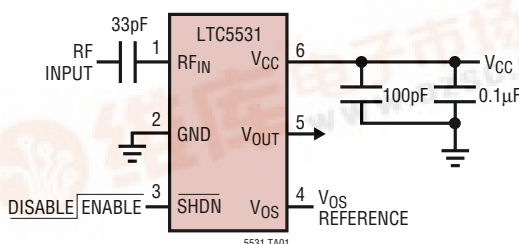
300MHz to 7GHz RF Power Detector
