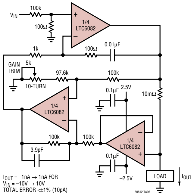
Precision Nanoamp Bidirectional Current Source
