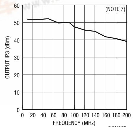
Equivalent Output IP3 vs Frequency
