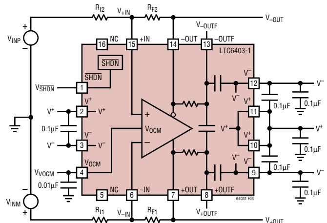
Figure 3. Real-World Application with Feedback Resistor Pair Mismatch
