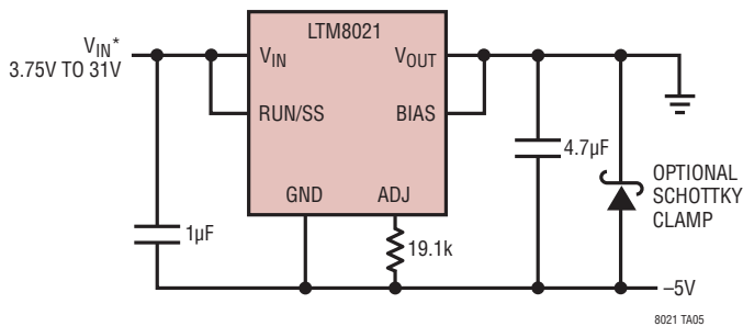
-5V Positive-to-Negative Converter
