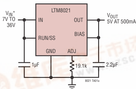
7V IN to 36V IN , 5V/500mA \mu Module Regulator
