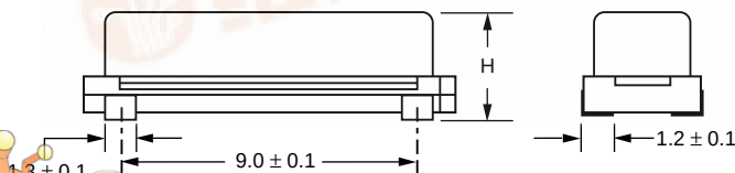
Figure 1) CSM-4A - Top, Side and End views
