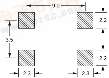
Figure 3) Land Pattern
