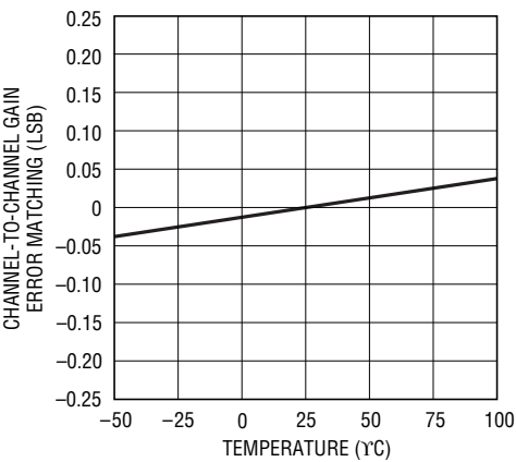
LTC1854 Channel-to-Channel Gain Error Matching vs Temperature
