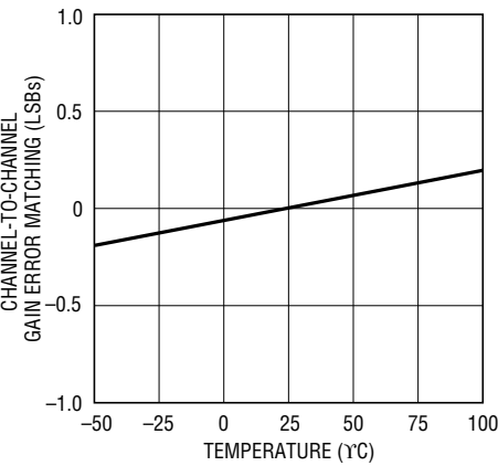
LTC1856 Channel-to-Channel Gain Error Matching vs Temperature
