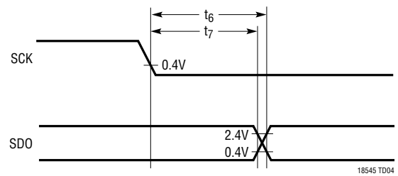
t_6 (Delay Time, \text{SCK} \square to SDO Valid) t_7 (Time from Previous Data Remains Valid After \text{SCK} \square )
