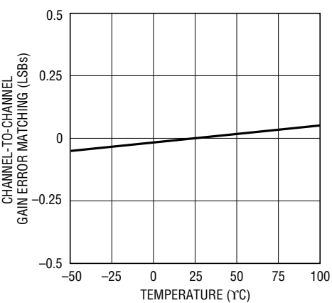
LTC1855 Channel-to-Channel Gain Error Matching vs Temperature
