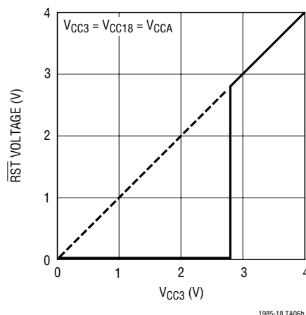
Resistor on \overline{RST} Output to Ground Ensures \overline{RST} Valid to V_{CC} = 0V
