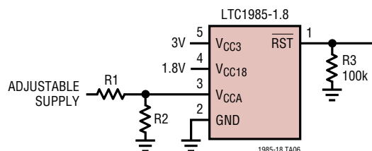
Resistor on \overline{RST} Output to Ground Ensures \overline{RST} Valid to V_{CC} = 0V
