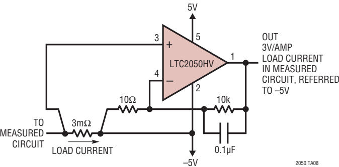
Low-Side Power Supply Current Sensing
