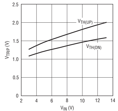
\overline{\text{SHDN}} Input Voltage Thresholds vs V_{\text{IN}}
