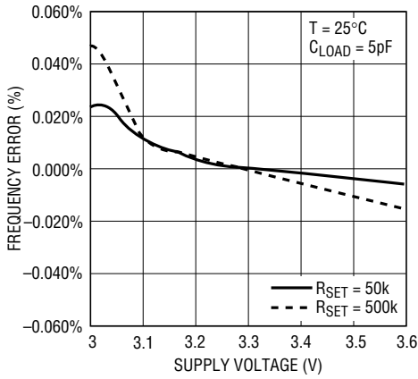
Typical Frequency Error vs Power Supply Voltage
