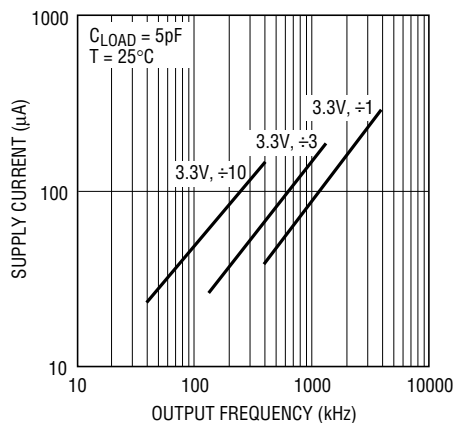
Figure 9. Supply Current vs Frequency over DIV Settings
