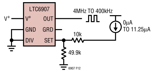
Figure 12. Current Controlled Oscillator
