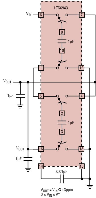
Divide by 3
