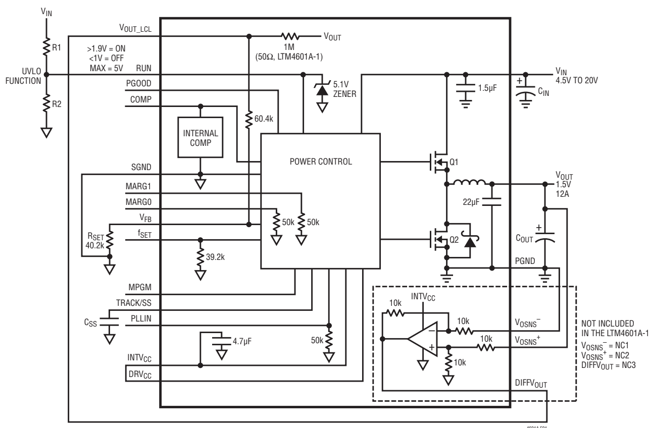
Figure 1. Simplified LTM4601A/LTM4601A-1 Block Diagram
