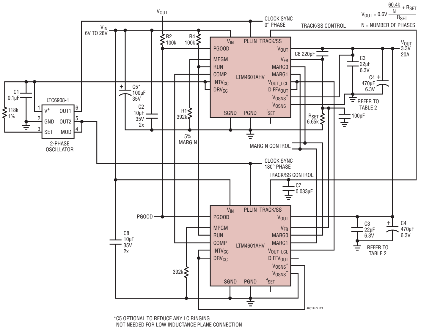
Figure 21. 2-Phase Parallel, 3.3V at 20A Design
