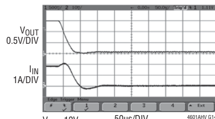
Short-Circuit Protection, I_{OUT} = 12\text{A}
