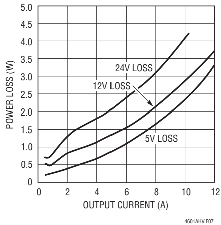
Figure 7. 24V IN and 1.5V Power Loss
