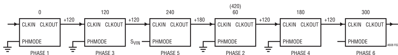
Figure 2. 6-Phase Operation
