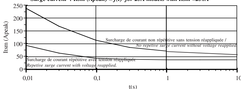
Fig.3 Surchage de courant : Itsm (Apeak) = f(t) pour modèle 25A(Itsm=230A) Surge current : Itsm (Apeak) = f(t) for 25A models with Itsm =230A
