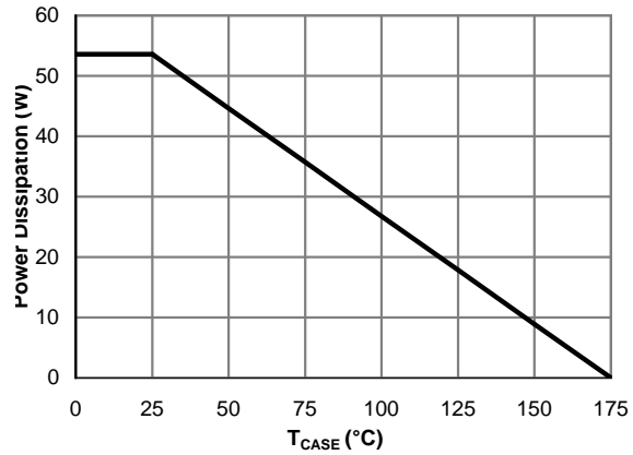
Figure 11: Power De-rating (Note B)
