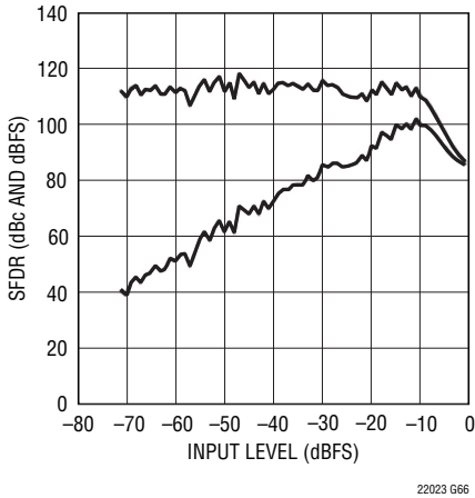
LTC2202: SFDR vs Input Level, f_{IN} = 70.1\text{MHz} , \text{PGA} = 0 , Dither "On"
