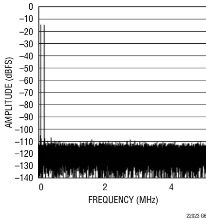
LTC2202: 32K Point 2-Tone FFT, f_{IN} = 60.2\text{MHz} and 70.1\text{MHz} , -15\text{dBFS} , \text{PGA} = 0
