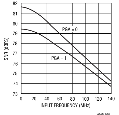
LTC2202: SNR vs Input Frequency
