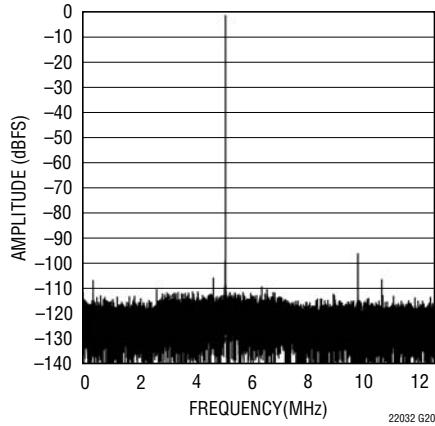
LTC2203: 32K Point FFT, f_{IN} = 30\text{MHz} , -1dBFS, PGA = 1
