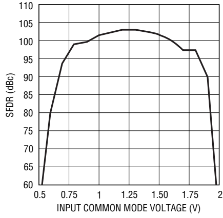
LTC2202: SFDR vs Input Common Mode Voltage, f_{IN} = 5\text{MHz} , -1dBFS, PGA = 0
