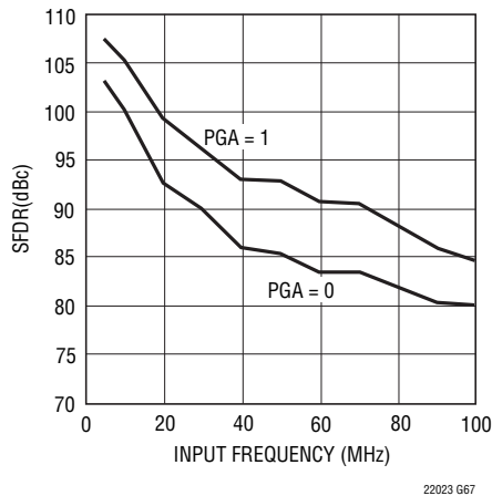
LTC2202: SFDR (HD2 or HD3) vs Input Frequency
