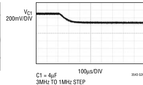
PLL Operation
