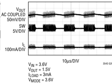
Pulse Skip Operation
