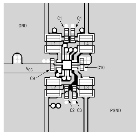
Figure 4. LTC3544 Suggested Layout
