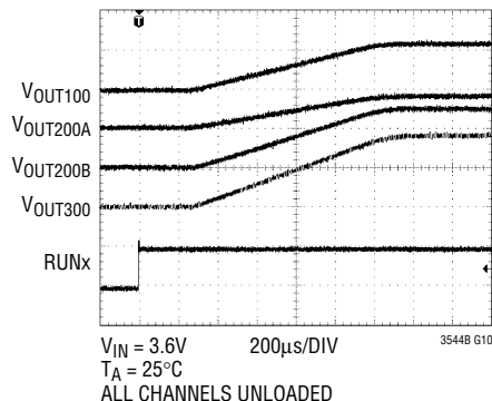
Figure 1. Regulator Soft-Start
