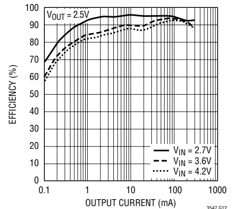
Efficiency vs Load Current ( V_{OUT} = 2.5V )
