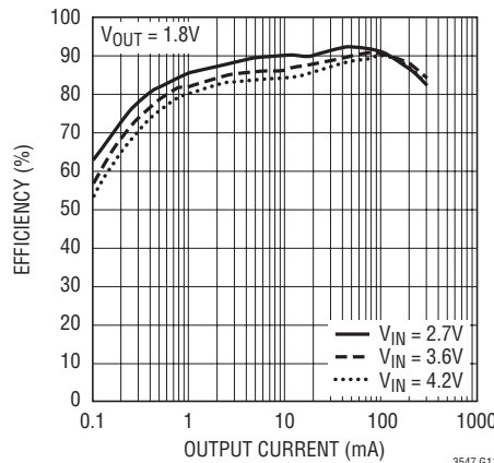
Efficiency vs Load Current ( V_{OUT} = 1.8V )
