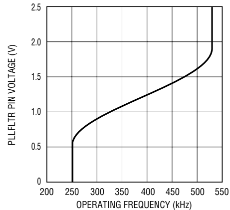
Figure 5. PLLFLTR Pin Voltage vs Frequency
