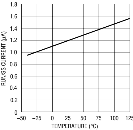
RUN/SS Current vs Temperature
