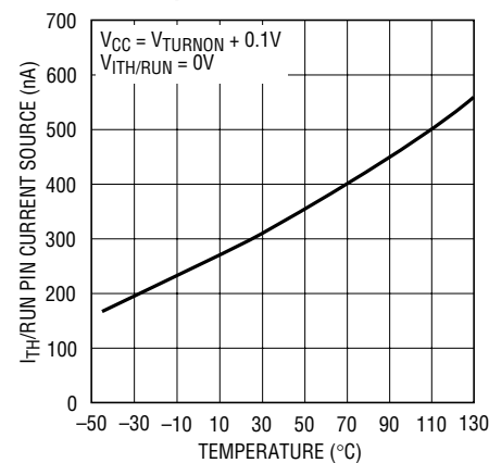
I_{TH}/\text{RUN} Start-Up Current Source vs Temperature
