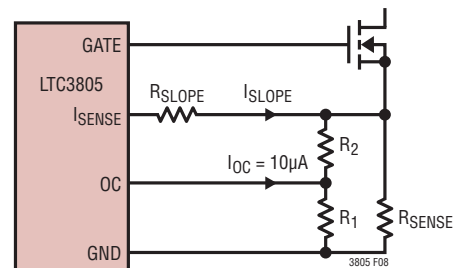
Figure 8. Circuit to Increase the Overcurrent Threshold for Large Switch Currents
