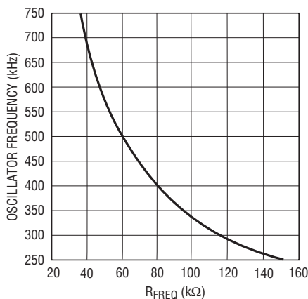
Figure 7. Relationship Between Oscillator Frequency and Resistor Connected Between FREQ/PLLFLTR and GND
