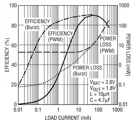
Buck Efficiency vs Load Current ( V_{OUT} = 1.8V )
