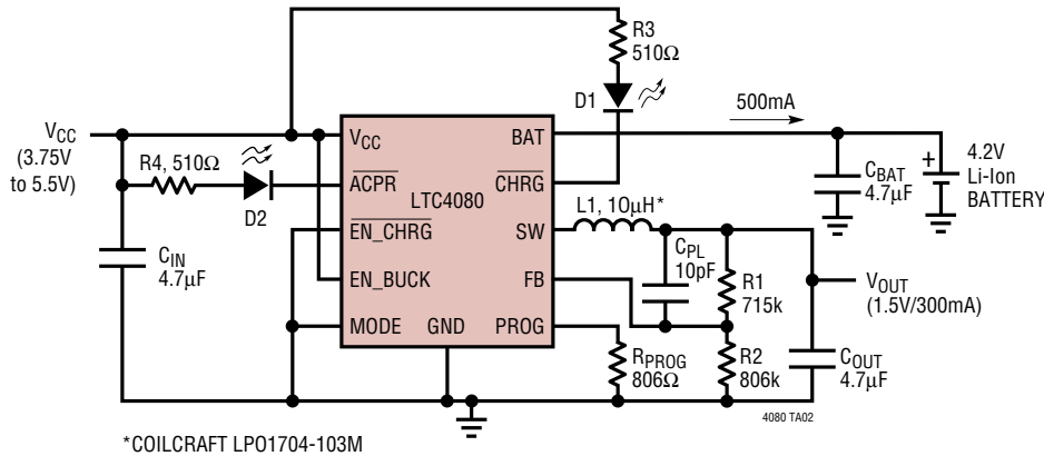
Li-Ion Battery Charger with 1.5V Buck Regulator
